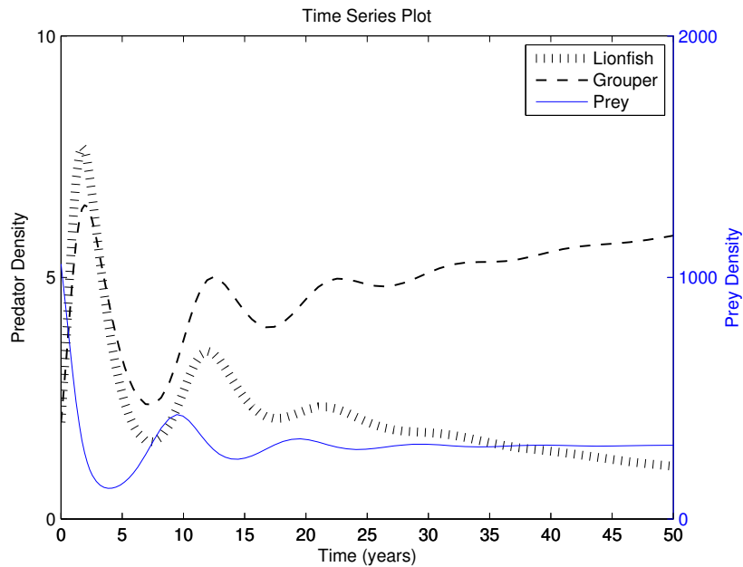
FIGURE 12. Low initial predator density with b_2 = 0.0026885 , d_1 = 0.3 , d_2 = 0.22 . This may reflect the Bahamas, where lionfish may be able to be eradicated if they are harvested much faster than grouper.
