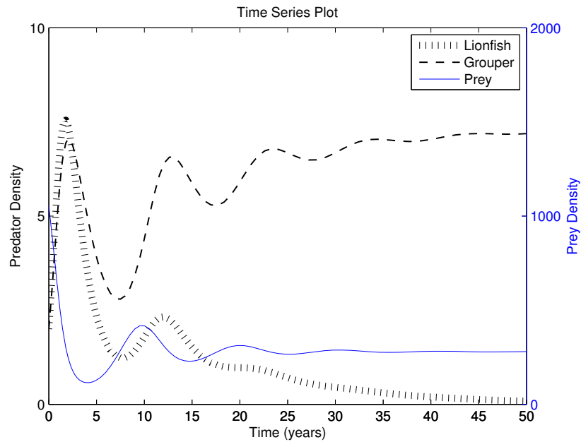
FIGURE 14. Low initial predator density with d_1 = 0.22 , b_2 = .0026885 , d_2 = 0.3 . This reflects the same scenario as in Figure 13 but with slight harvesting on lionfish. This is enough to drive the population to extinction over time.
