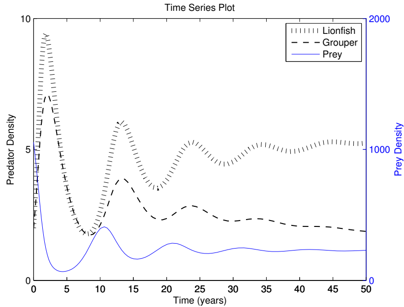
FIGURE 13. Low initial predator density with b_2 = 0.0026885 , d_1 = 0.22 , d_2 = 0.22 . This may simulate the eastern coasts of the United States, where, at the initial stages of the invasion, harvesting of Nassau grouper was banned due to overfishing. With no harvesting on grouper, the lionfish can still invade, but coexistence is possible.
