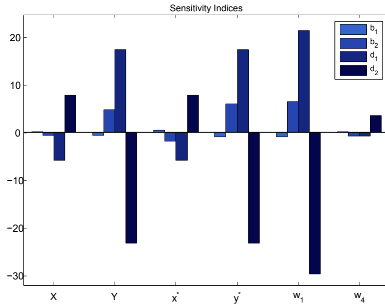
FIGURE 15. Sensitivity analysis of stability conditions for E_2 and E_3 , the lionfish and grouper components of the coexistence equilibrium, and the stability condition for the coexistence equilibrium.
