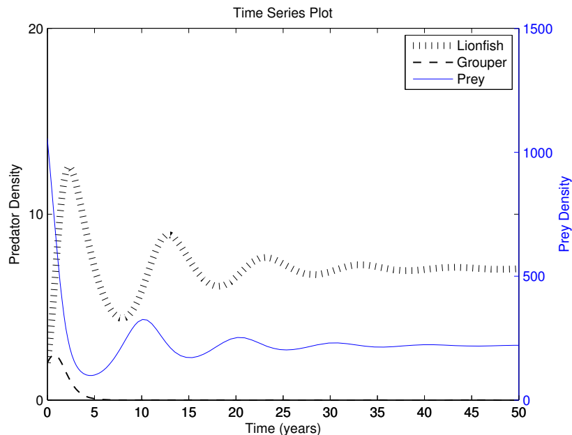
FIGURE 9. Low initial predator density with no harvesting and low predation on lionfish ( d_1 = 0.22 , b_2 = .0026885 ), and moderate fishing on grouper ( d_2 = 0.6 ). This may reflect the Bahamas with grouper overfishing. Lionfish invasion and grouper extinction occur rapidly.
