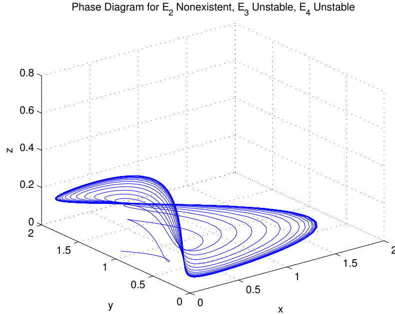
FIGURE 5. A stable limit cycle emerges when E_4 becomes unstable. As before, E_1 is unstable, E_2 is nonexistent, and E_3 is unstable. Parameters used: A_1 = 1.0, A_2 = 5.0, A_3 = 0.1, A_4 = 3.0, A_5 = 2.0, A_6 = 1.0, A_7 = 3.0, A_8 = 0.1 .
