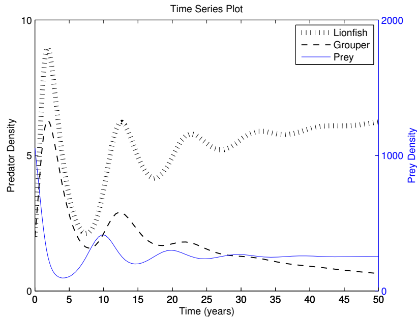
FIGURE 11. Low initial predator density with b_2 = 0.0026885 , d_1 = 0.25 , d_2 = 0.2416 . This may reflect the Bahamas, where coexistence is possible with low harvesting of both species.
