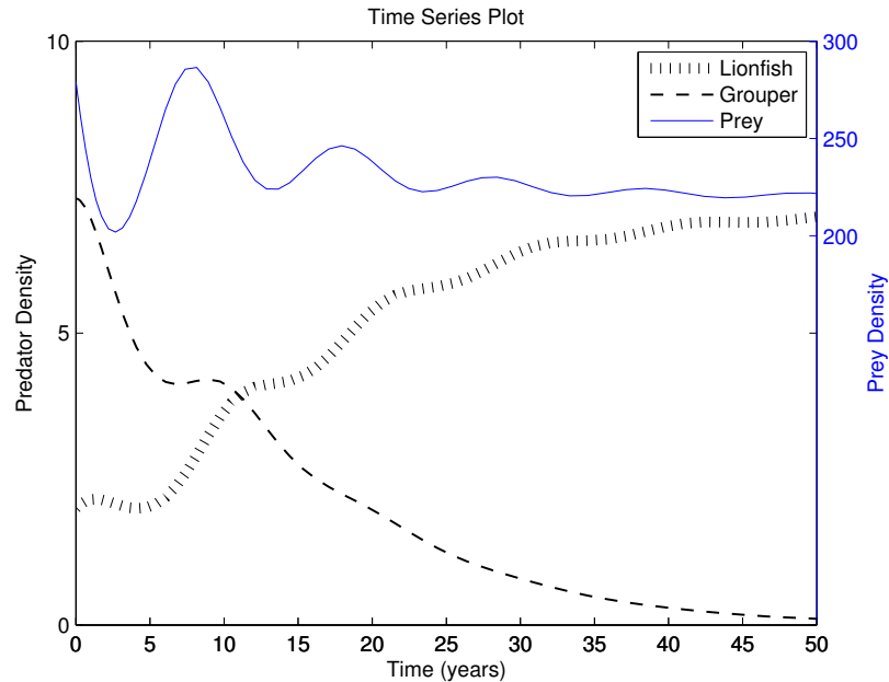
FIGURE 8. Low initial lionfish density with no IGP ( b_1 = b_2 = 0 ) and no harvesting ( d_1 = d_2 = 0.22 ). This may simulate ECLSP starting at the beginning of the lionfish invasion, assuming grouper never learn to consume lionfish and lionfish are negligible consumers of grouper.
