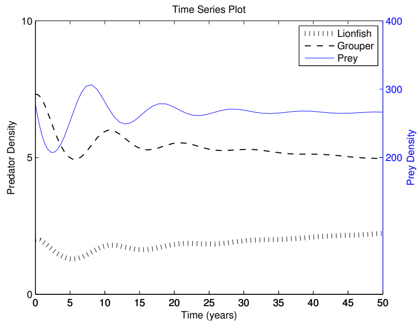
FIGURE 7. Low initial lionfish density with minimum calculated IGP ( b_2 = 0.0026885 ), no harvesting on grouper ( d_2 = 0.22 ), and slight harvesting on lionfish ( d_1 = 0.25 ). This may simulate ECLSP if such harvesting is allowed.
