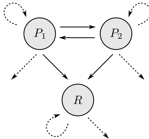
FIGURE 1. Conceptual model of general three-population model with symmetric intraguild predation. Solid lines represent predation dynamics (with arrows pointing towards prey); dotted loops represent fecundity and dotted lines represent mortality (natural deaths and harvesting).
