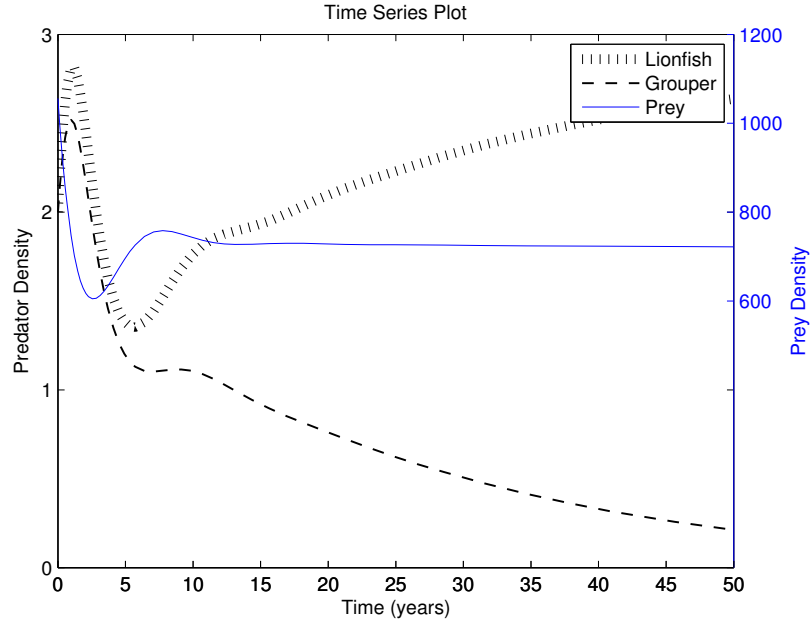
FIGURE 10. Low initial predator density with b_2 = 0.0026885 . This may reflect the Bahamas, where despite high lionfish removal ( d_1 = 0.72 ), continued grouper harvesting ( d_2 = 0.6 ) allows lionfish to be successful. Notice that despite the initial decrease in lionfish population, they are still able to persist as the grouper population declines.
