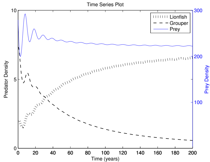
FIGURE 6. Low initial lionfish density with maximum estimated IGP ( b_2 = 0.0037515 ) and no harvesting ( d_1 = d_2 = 0.22 ). This may simulate ECLSP assuming grouper consistently predate on lionfish. IGP greatly slows the rate of lionfish takeover compared to Figure 8 but does not stop it.
