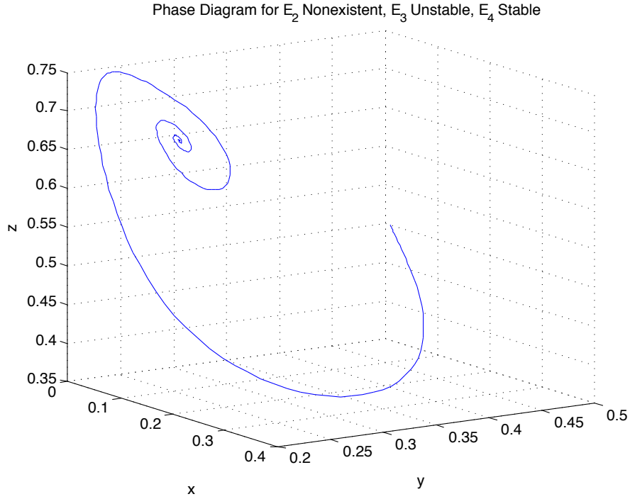
FIGURE 4. A solution spirals towards E_4 when stable. In this case, E_1 is unstable, E_2 is nonexistent, and E_3 is unstable. Parameters used: A_1 = 1.0, A_2 = 5.0, A_3 = 0.1, A_4 = 2.0, A_5 = 0.2, A_6 = 1.5, A_7 = 2.0, A_8 = 0.1 .
